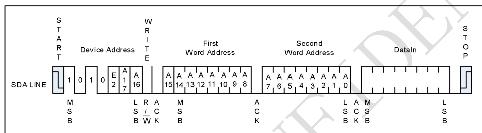
Figure 5-1 Byte Write
