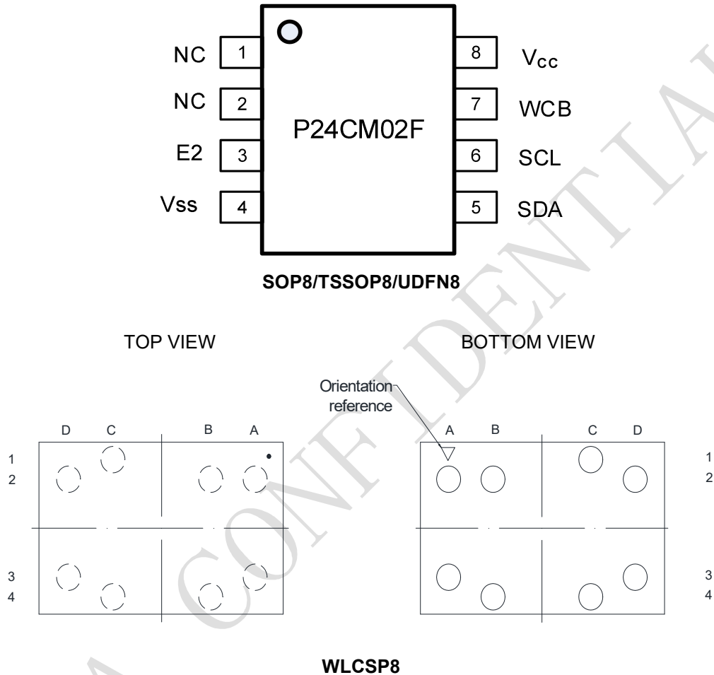
Figure 1-1 Pin Configuration
